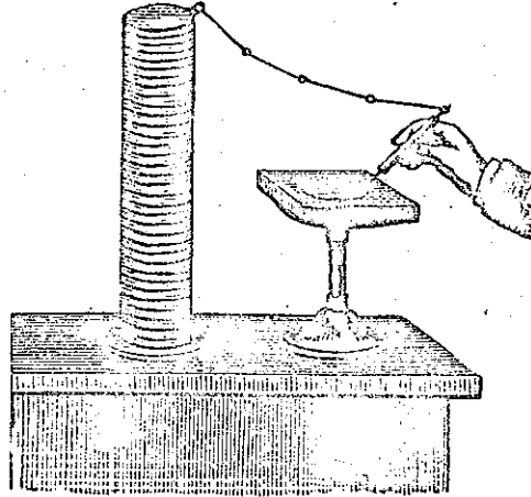
Romagnosi's experiment: Contact between one "pole" of the pile and the compass needle resulted in deflection of the latter. (After Fahie)(1)
