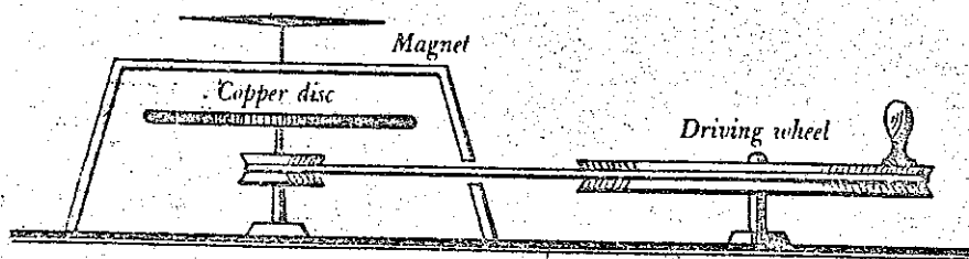
FIGURE 2. The Arago rotation-experiment, disclosed 7 March 1825, by which a magnetic needle is made to drag after a revolving copper disc. (From B. Dibner, Faraday discloses electro-magnetic induction , Burndy Library, 1949.)
